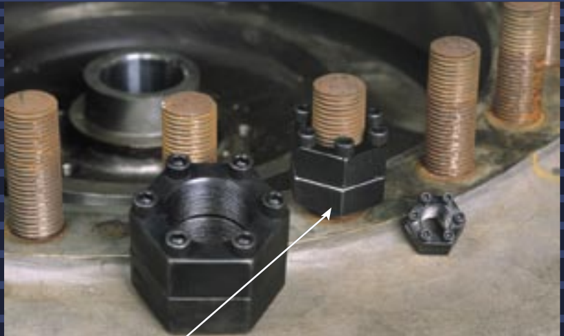
Threads on close to base reducing side load when removing stud.
