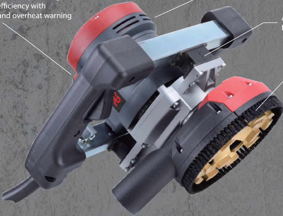
Tool-free sliding cover for edge grinding
